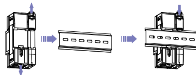
Figure 4-1 Mounting Wi-BR
